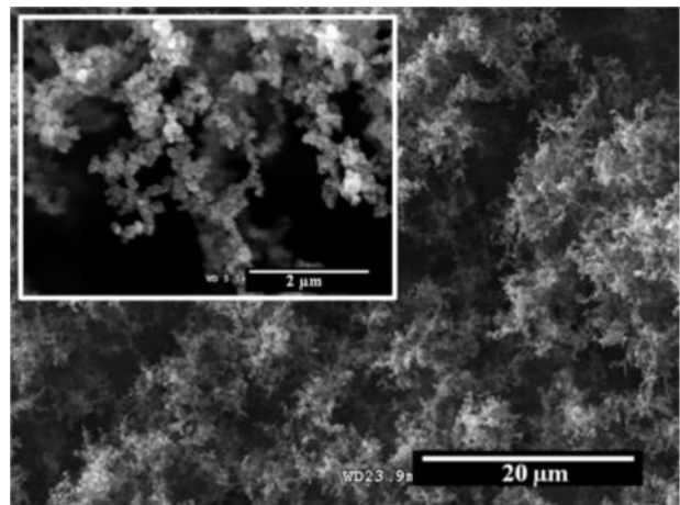
Figure 1. Upper view SEM micrograph of a dry ES deposit formed by carbon nanoparticles.
